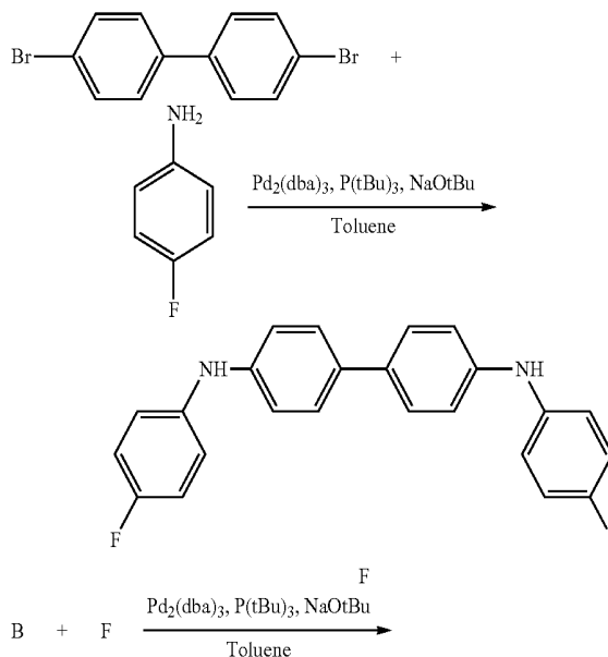
Reaction Scheme 5
