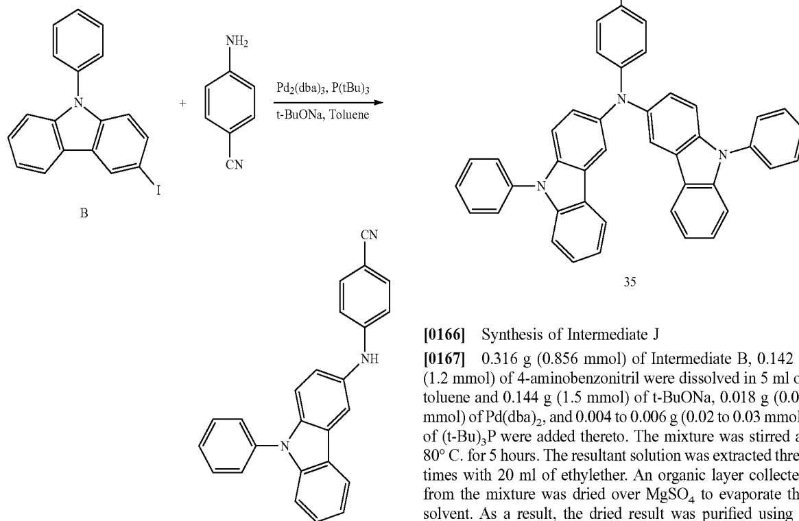
Reaction Scheme 8
