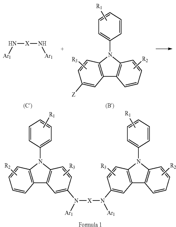
Reaction Scheme 1
