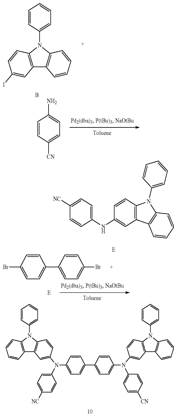
Reaction Scheme 4
